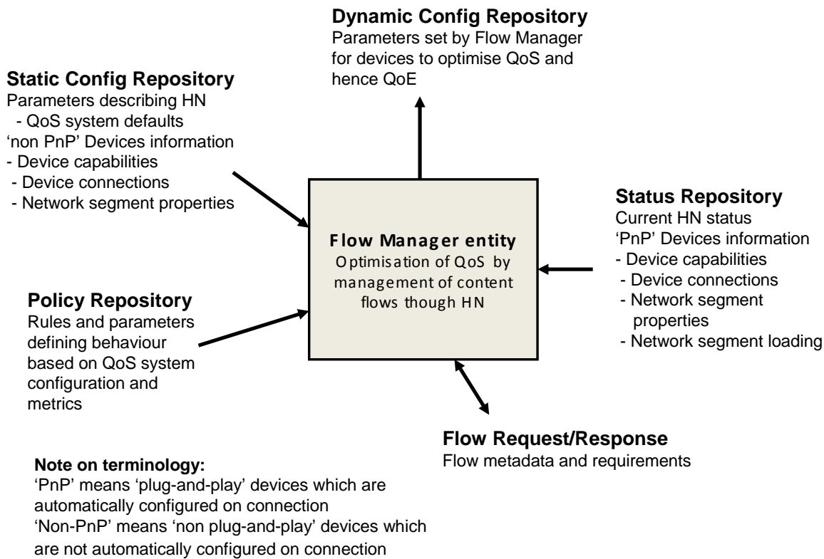
Figure 5: Operation of Flow Manager Entity
