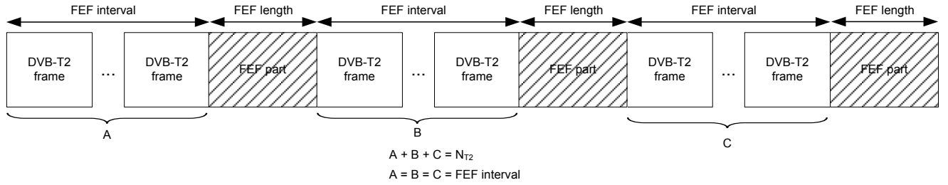
Figure 35: The super-frame, including T2-frames and FEF parts
