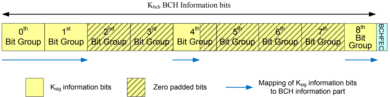
Figure 31: Example of Shortening of BCH information part
