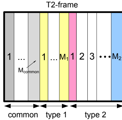
Figure 41: Allocation of M_{common} common PLPs, M_1 data PLPs of type1 and M_2 data PLPs of type 2 transmitted in one T2-frame
