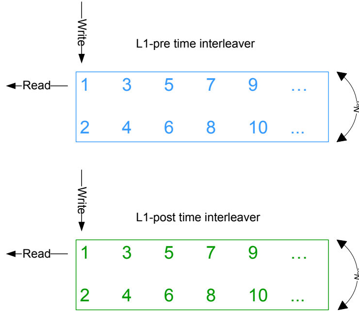
Figure 40: P2 time interleaver.
