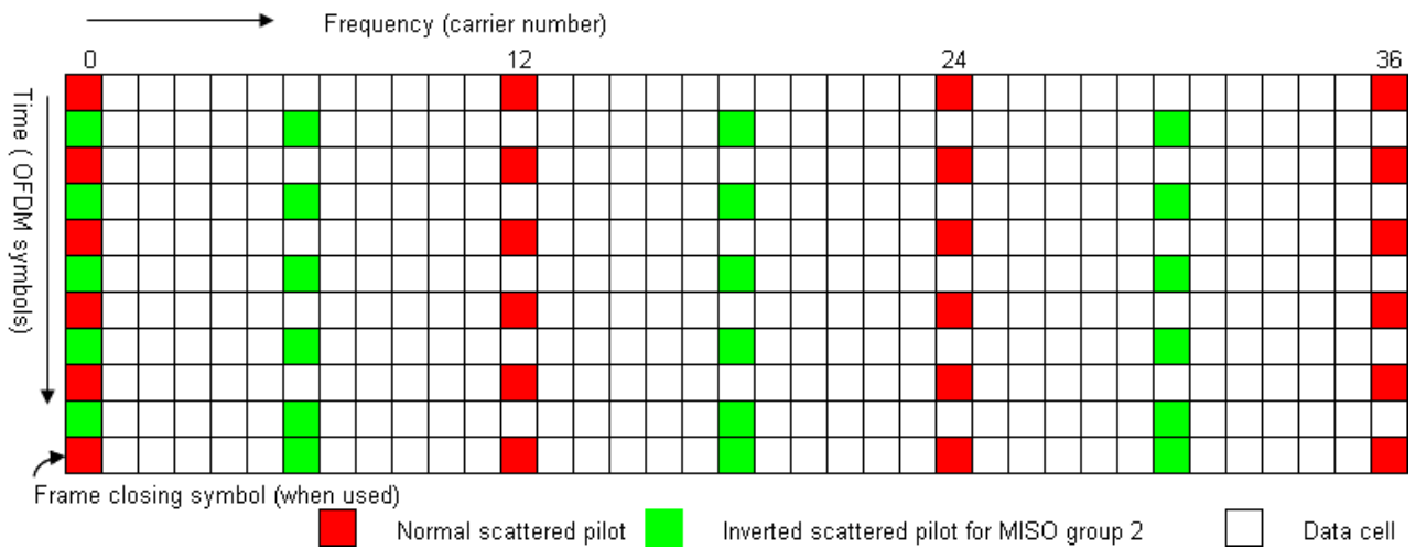
Figure J.10: Scattered pilot pattern PP2 (MISO)
