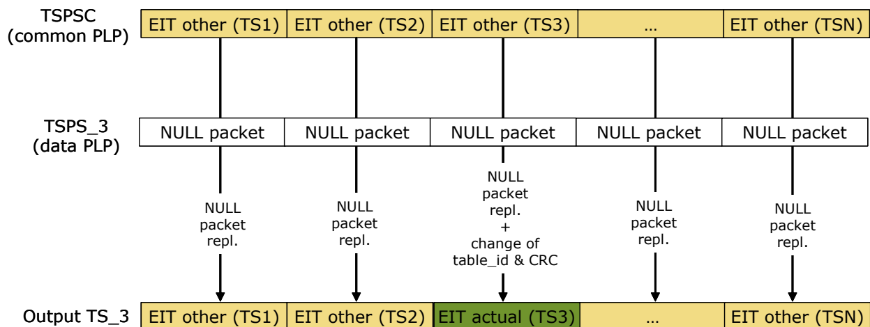
Figure D.6: Receiver operation to re-combine of TSPS and TSPSC into output TS for EIT
