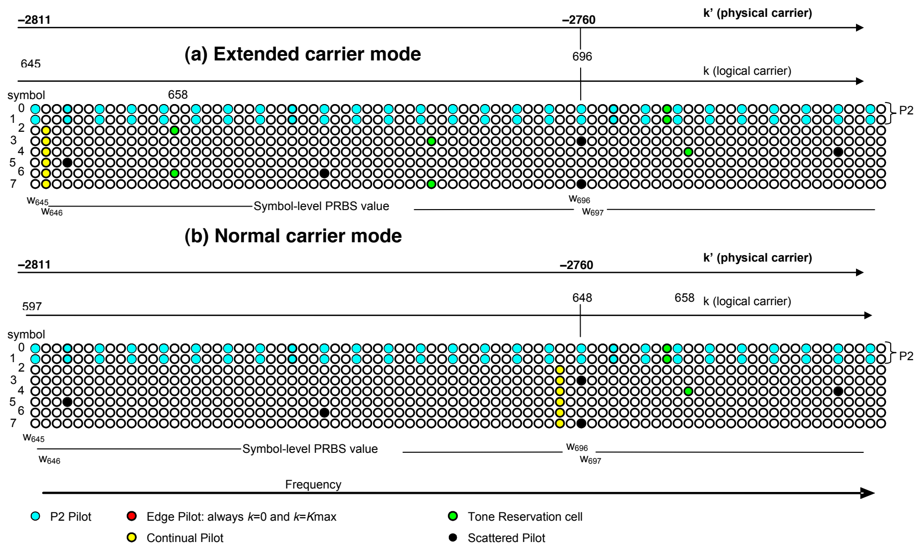
Figure J.18: Example of pilot and TR cells in extended and normal carrier mode (8K PP7)
