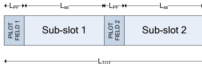
Figure 5.23: Slot pilot insertion
