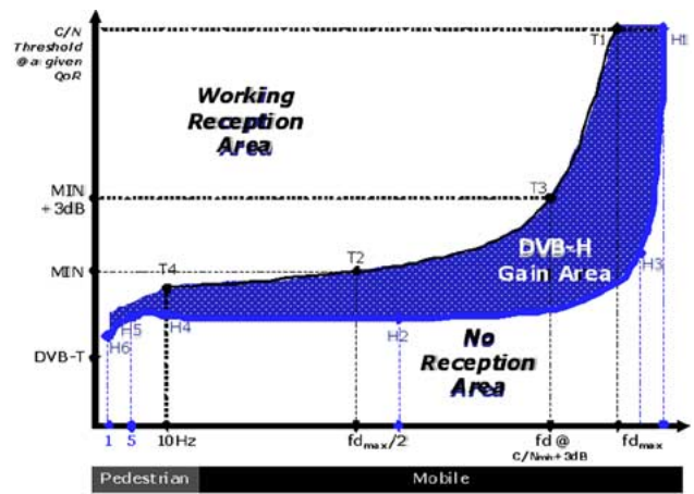
Fig. 8. C/N versus Doppler for receivers in motion.
