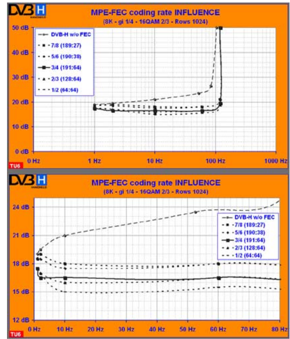
Fig. 11. MPE-FEC coding rate influence in 16QAM 2/3.
