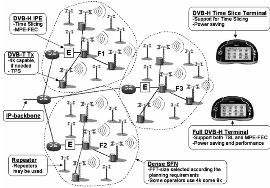
Fig. 15. A dedicated DVB-H network.
