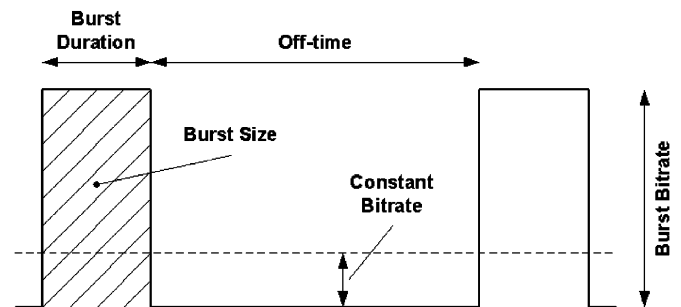
Fig. 4. Principle of time slicing.
